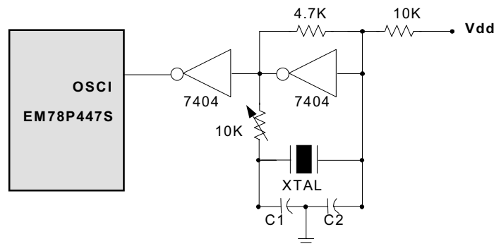
Fig. 13 Crystal/Resonator-Parallel Mode Circuit
