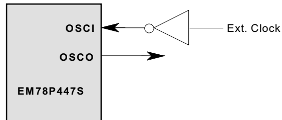
Fig. 10 Crystal/Resonator Circuit
