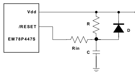
Fig. 15 External Power-Up Reset Circuit
