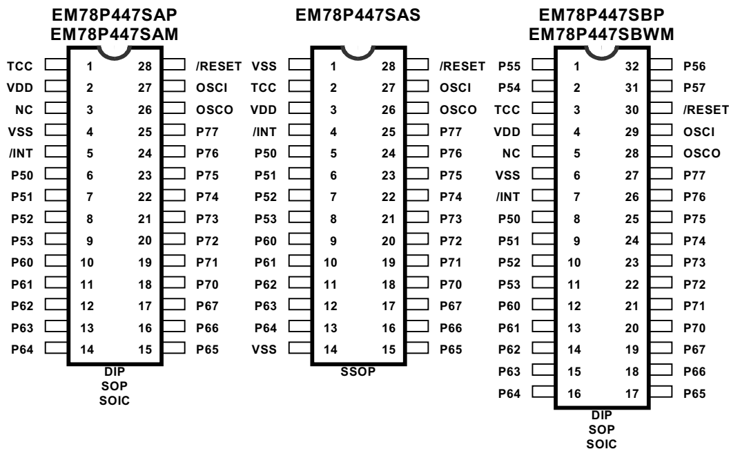
Fig. 1 Pin Assignment
