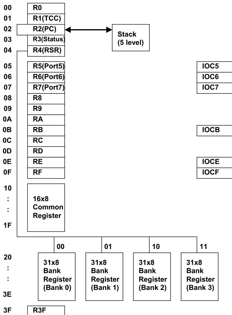
Fig. 4 Data Memory Configuration
