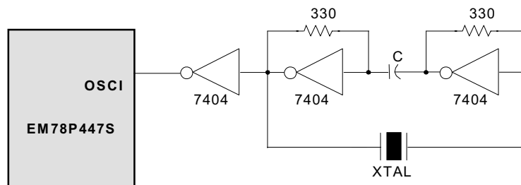
Fig. 12 Crystal/Resonator-Series Mode Circuit
