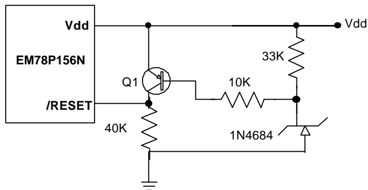
Fig. 17 Circuit 1 for the Residue Voltage Protection
