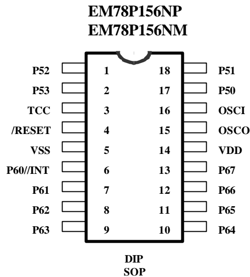
Fig. 1 Pin Assignment
