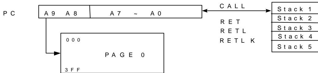
Fig. 3 Program Counter Organization
