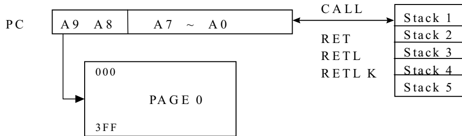
Fig. 3 Program Counter Organization
