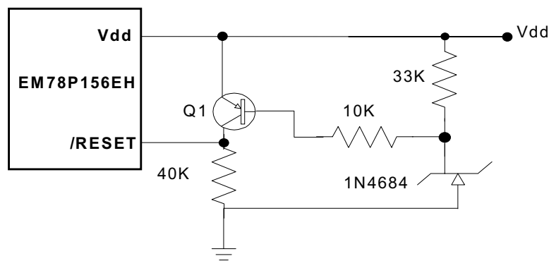
Fig. 17 Circuit 1 for the Residue Voltage Protection
