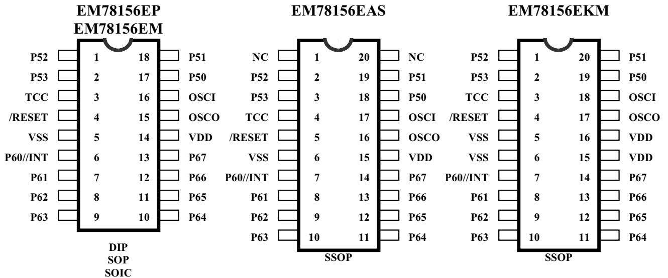
Fig. 1 Pin Assignment
