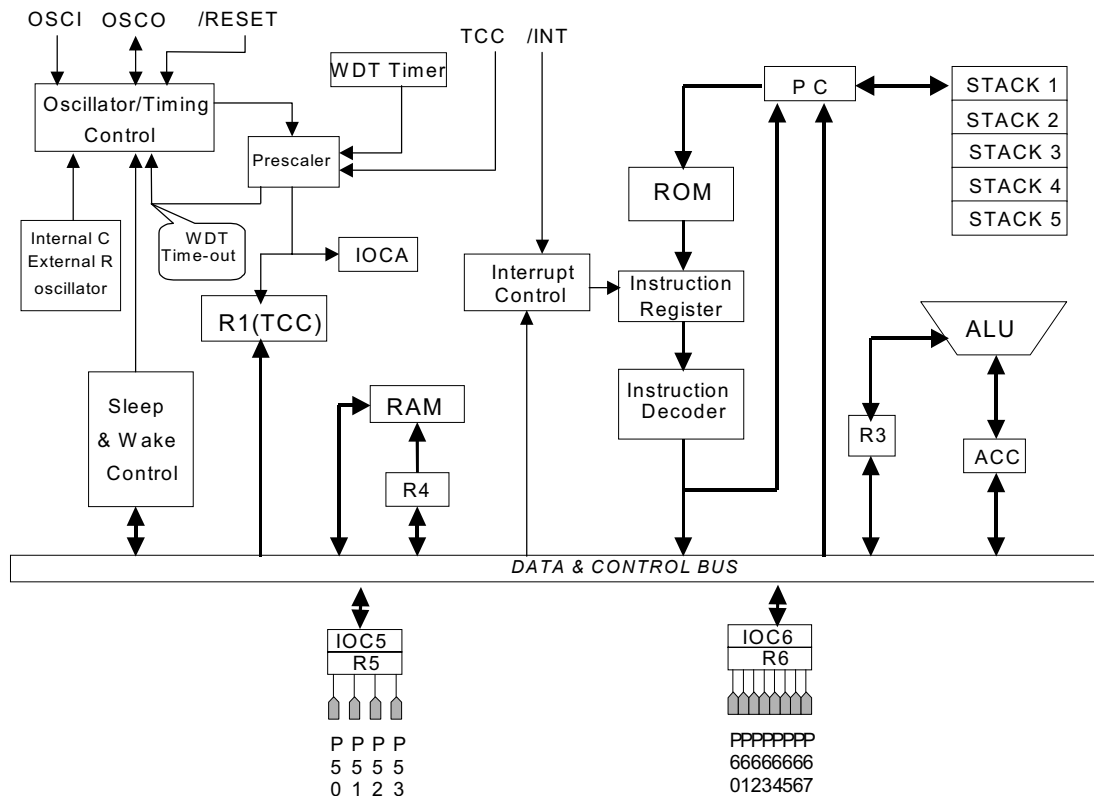
Fig. 2 Function Block Diagram
