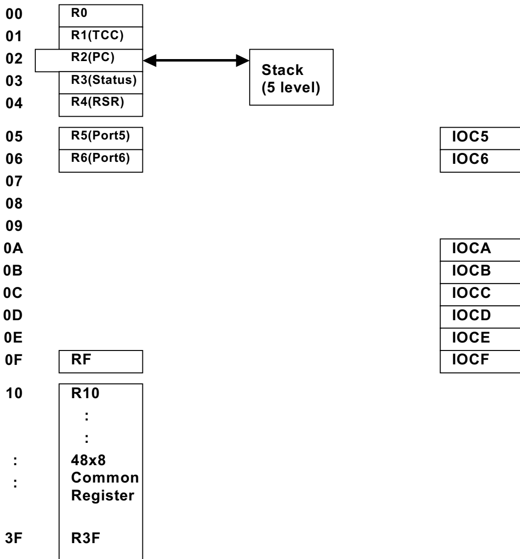
Fig. 4 Data Memory Configuration
